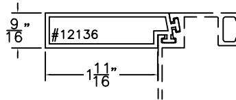
1 \frac{11}{16} " TUBE EXTENDER
